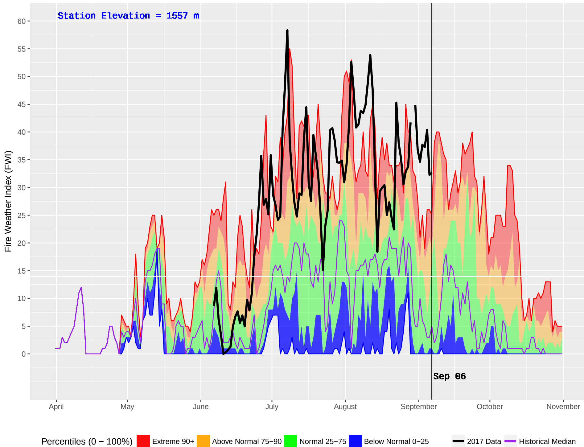
SKOONKA (1024) : Historical (2008–2016) and Current (2017) Noon Fire Weather Index (FWI)
