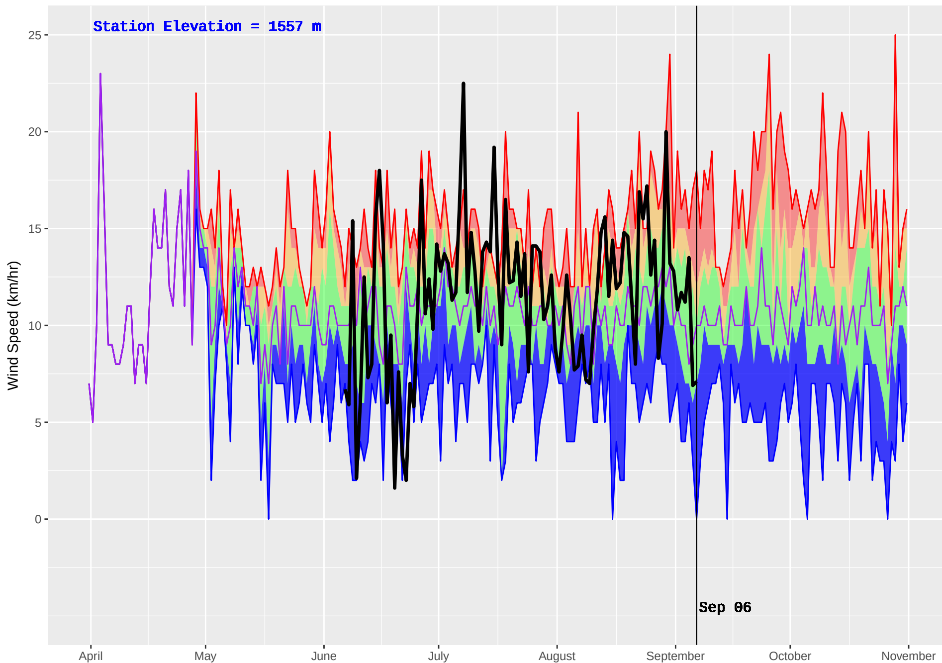
SKOONKA (1024) : Historical (2008–2016) and Current (2017) Noon Wind Speed
